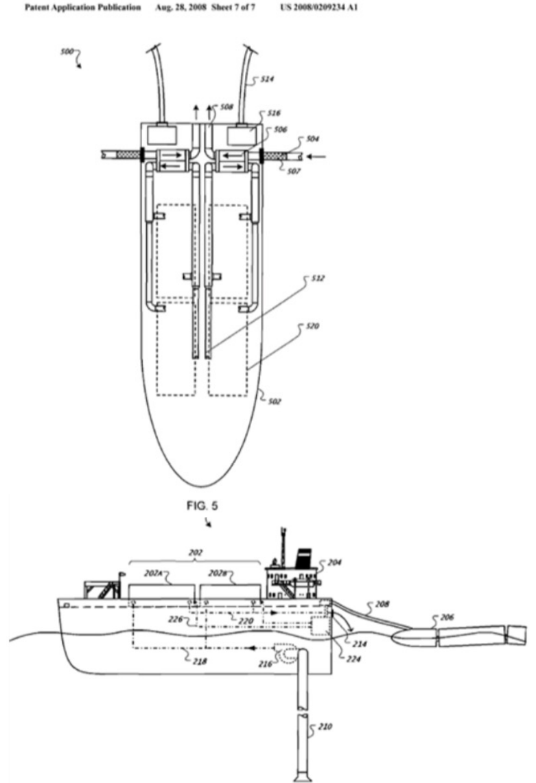
Google floating data centre design 2008
